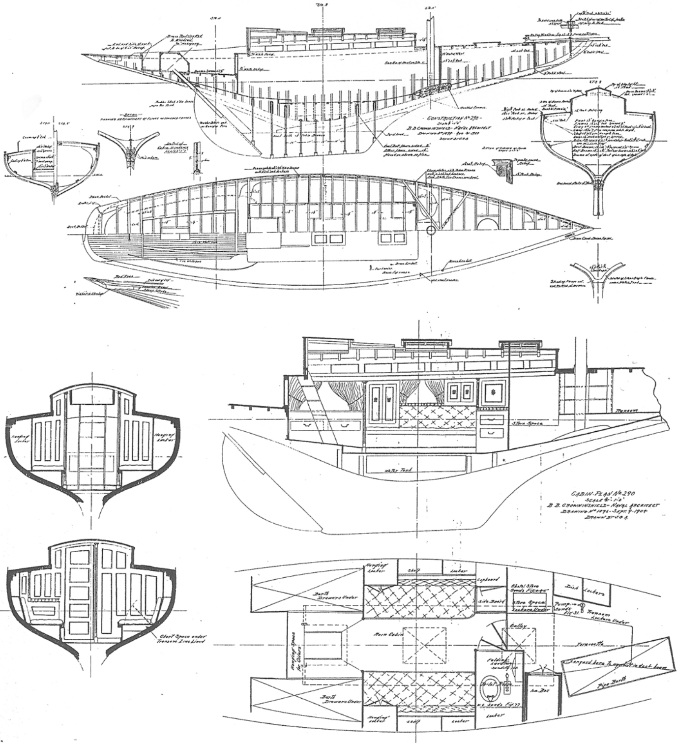
Cabin and Construction Plans of Cruising Sloop
